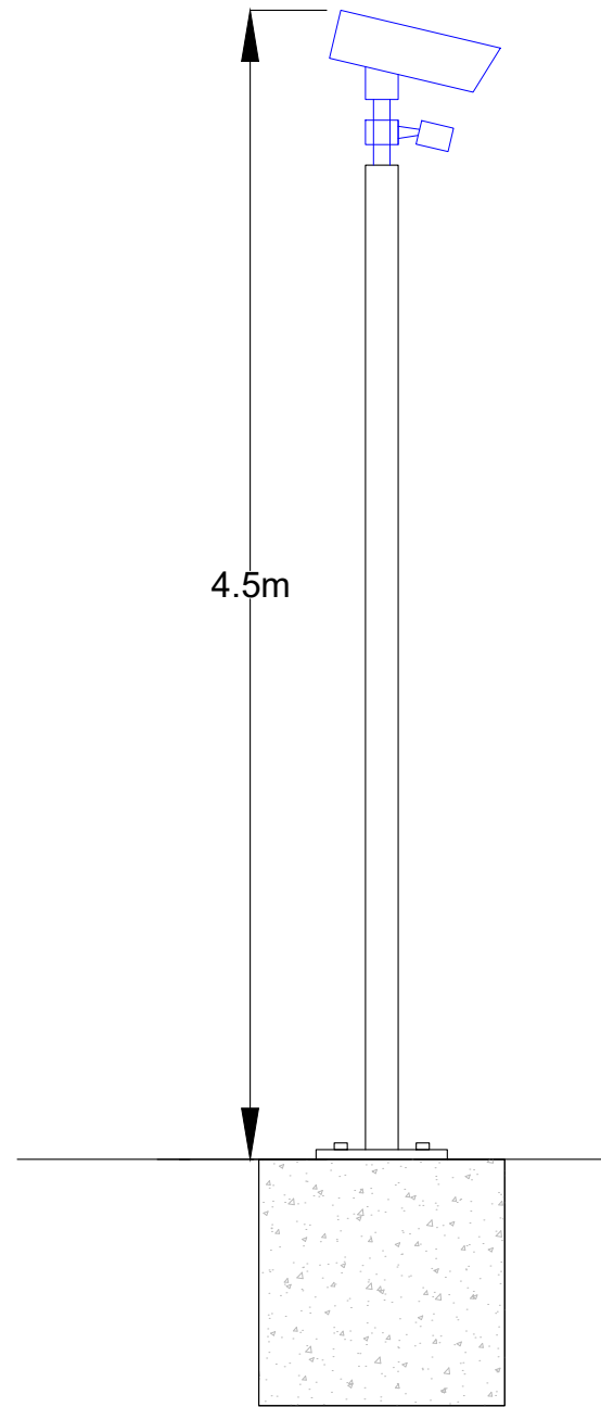
Typical Elevation
