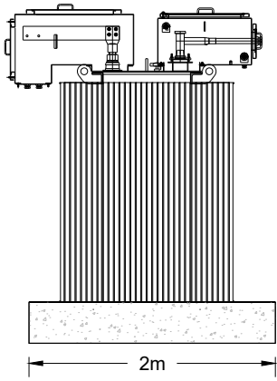
Side Elevation
