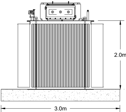
Front Elevation
