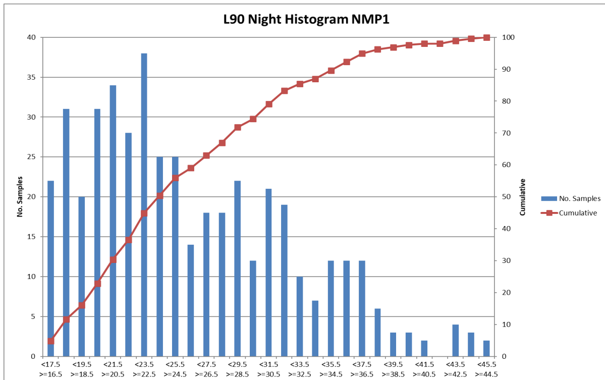
Graph 2: NMP1 Background, LA90, Analysis Night-time
